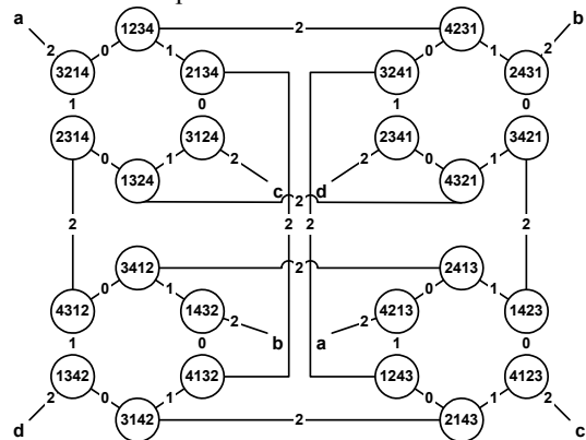
Figure 6. Star graph
